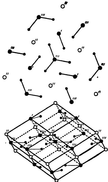
Structure of Calcite.
